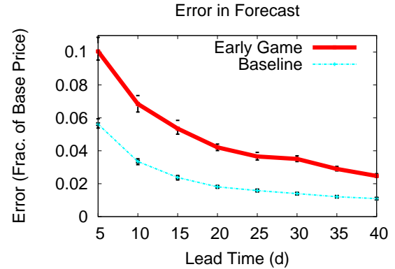
(b) Error of early segment component price prediction with baseline that used unlimited probes.
